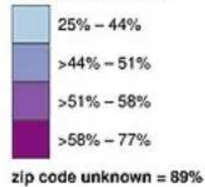
Percent of patients testing positive for COVID-19 by zip code in New York City as of March 31, 2020
